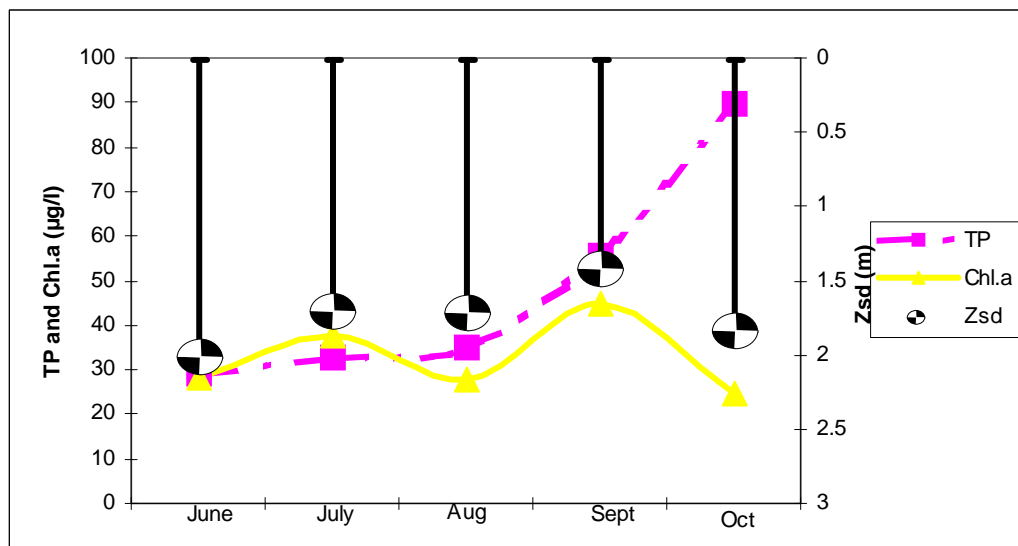
Figure 5- Eutrophication Data in a Typical (Monthly Mean) Year for Copake Lake
