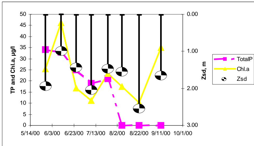
Figure 4. 2000 Eutrophication Data for Copake Lake
