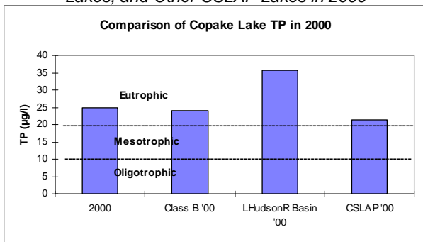
Figure 10. Comparison of 2000 Total Phosphorus to Lakes With the Same Water Quality Classification, Neighboring Lakes, and Other CSLAP Lakes in 2000
