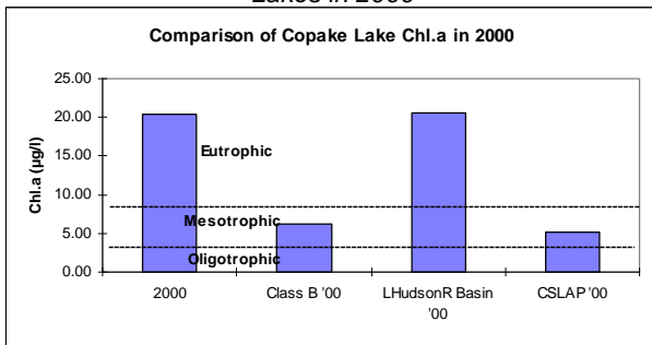
Figure 9. Comparison of 2000 Chlorophyll a to Lakes with the Same Water Quality Classification, Neighboring Lakes, and Other CSLAP Lakes in 2000
