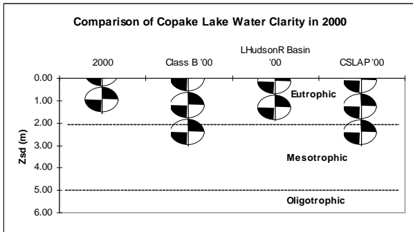
Figure 8. Comparison of 2000 Secchi Disk Transparency to Lakes With the Same Water Quality Classification, Neighboring Lakes, and Other CSLAP Lakes in 2000
